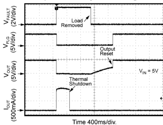
Thermal Shutdown MIC2026A: Output Reset by Removing Load
