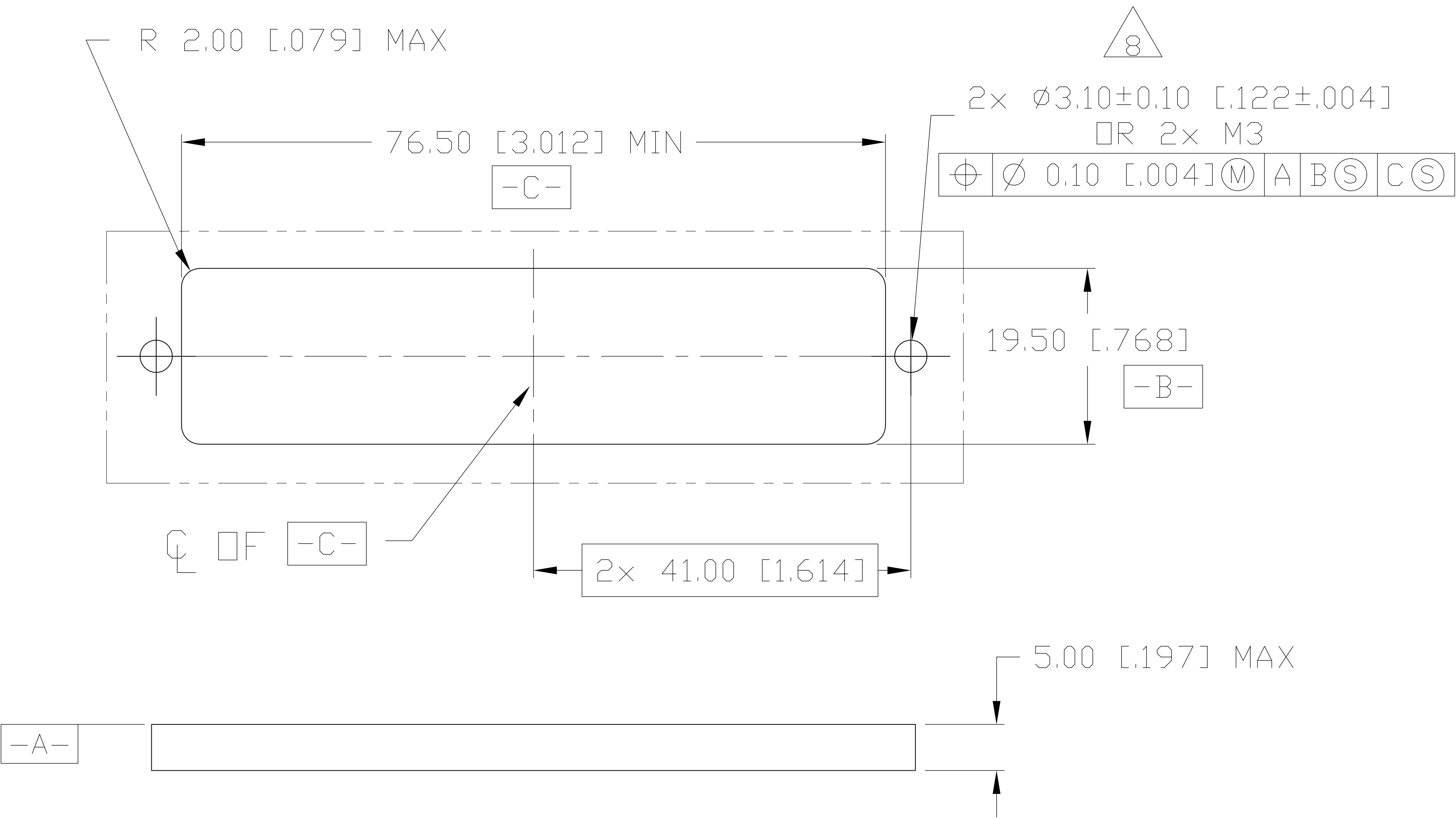
RECOMMENDED PANEL CUTOUT
