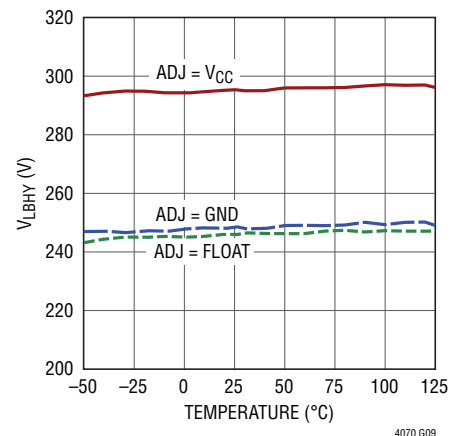
V_{LBHY} vs Temperature
