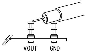
Figure 2. Measuring Output Ripple
