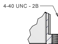
HARDWARE OPTION PF-0 (THREADED HOLES TO ACCEPT JACK POSTS)
