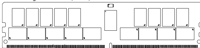
Figure 1: 288-Pin RDIMM (MO-309, R/C-B2)
