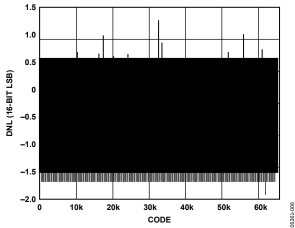
Figure 7. AD9779 Typical DNL
