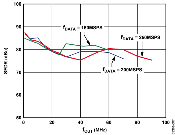
Figure 8. AD9779 In-Band SFDR vs. f_{OUT} , 1x Interpolation
