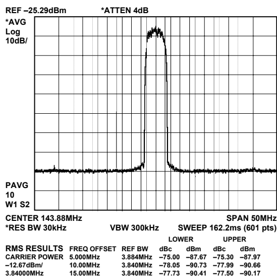
Figure 49. AD9776, Single Carrier WCDMA, 4x Interpolation, f_{\text{DATA}} = 122.88\text{ MSPS} , Amplitude = -3 dBFS
