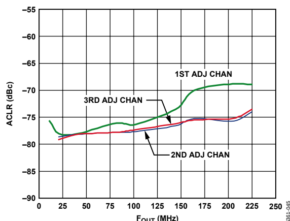
Figure 48. AD9776 ACLR, f_{\text{DATA}} = 122.88\text{ MSPS} , 4x Interpolation, f_{\text{DAC}}/4 Modulation
