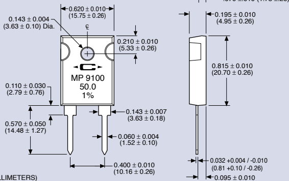
Figure 3 TO-247 Style MP9100
