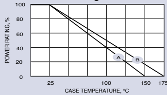
Derating Curve
