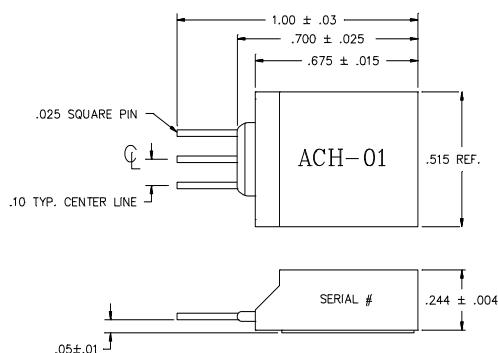
ACH-01-02 WITH PINS
