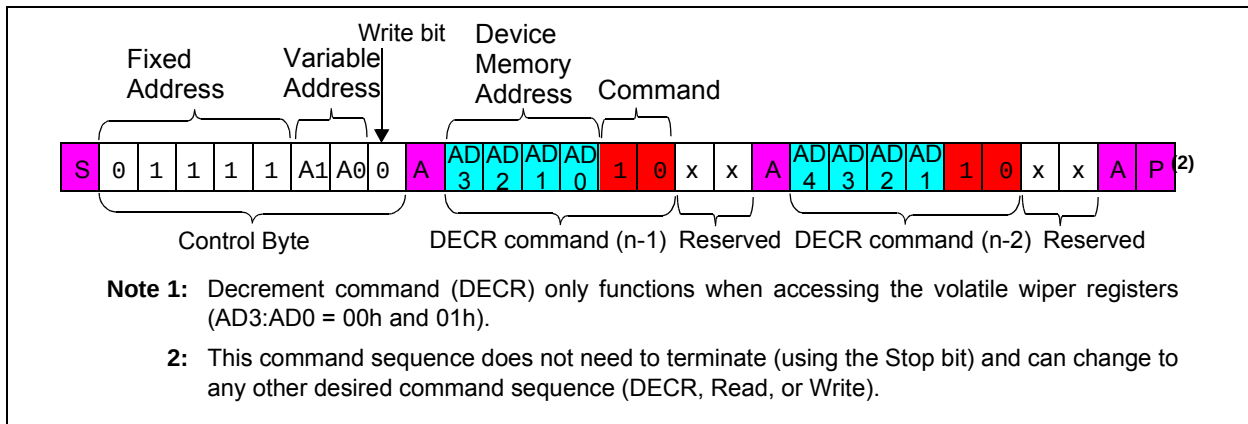
FIGURE 7-8: I²C Decrement Command Sequence.
