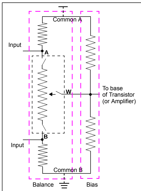
FIGURE 8-1: Example Application Circuit using Terminal Disconnects.
