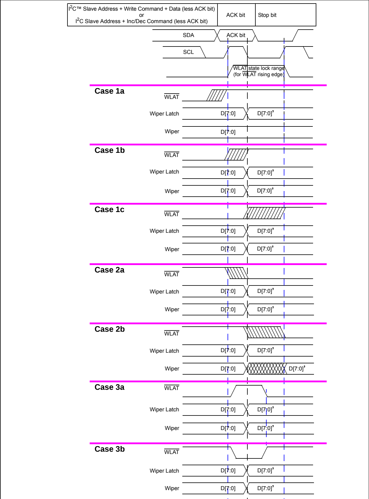
FIGURE 4-7: \overline{\text{WLAT}} Interaction with \text{I}^2\text{C} ACK Pulse
