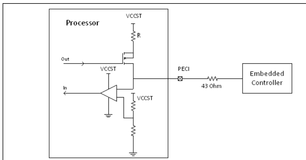
Figure 2-11. Example for PEGI EC Connection
