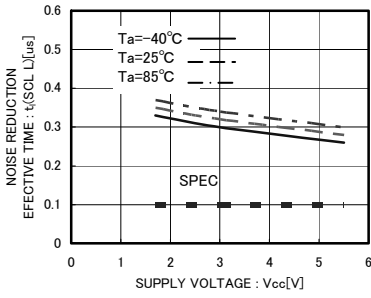
Fig.27 Noise reduction effective time t_I(SCL L)
