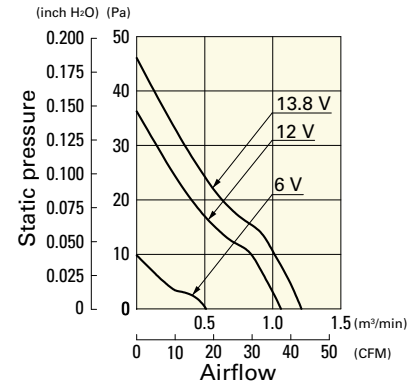
109R0812L401 With pulse sensor
