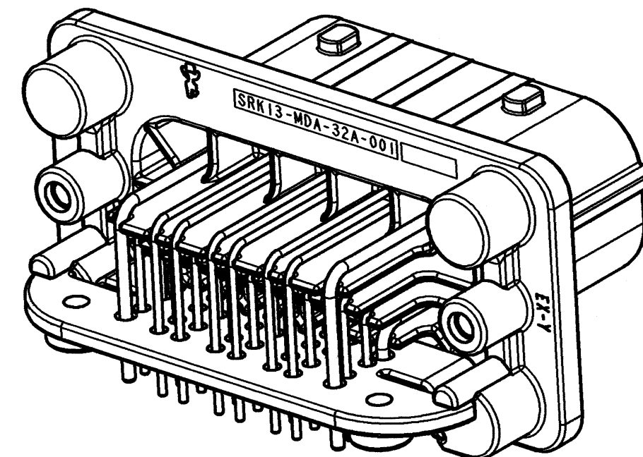
3D VIEW
