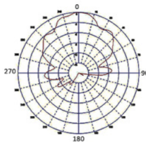
Typical Radiation Patterns - GPS/GNSS Element 1 Element 3: Typical E Plane Pattern
