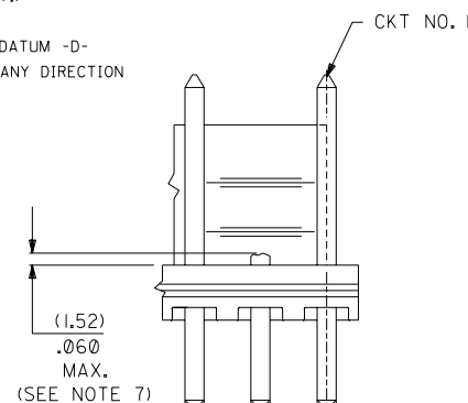
DETAIL A (OPTIONAL PIN CUT-OFF TYPE VOID)
