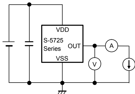
Figure 10 Test Circuit 3
