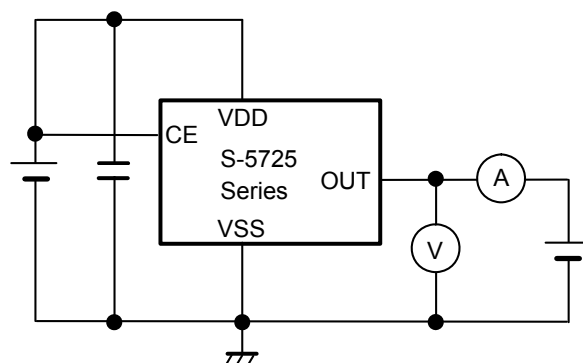
Figure 16 Test Circuit 4
