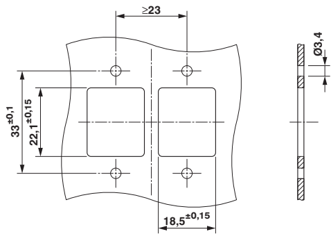
Drilling diagram
