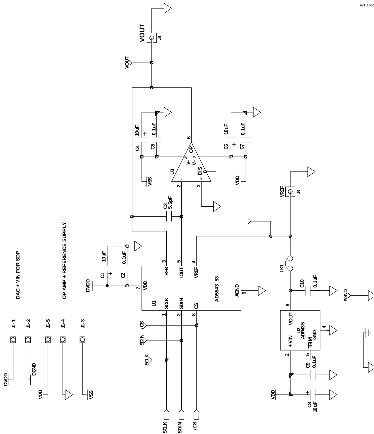
Figure 27. Schematic of AD5543/AD5553 Evaluation Board
