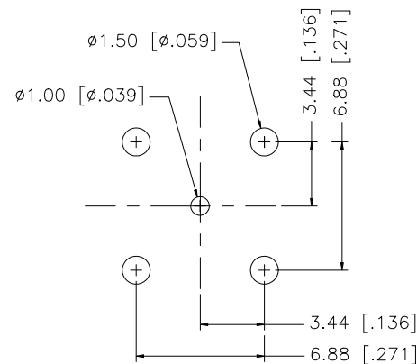
PCB MOUNTING HOLES
