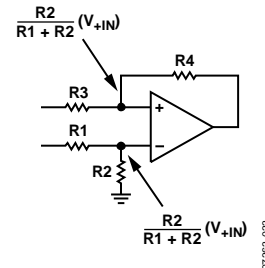
Figure 44. Voltage Division in the Difference Amplifier Configuration
