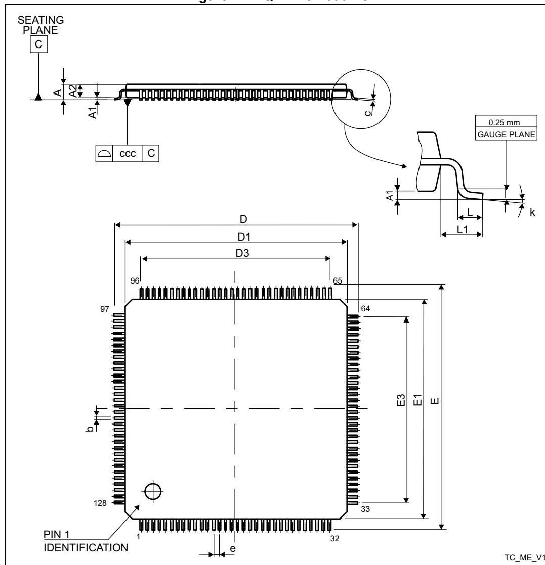
Figure 71. LQFP128 - outline
