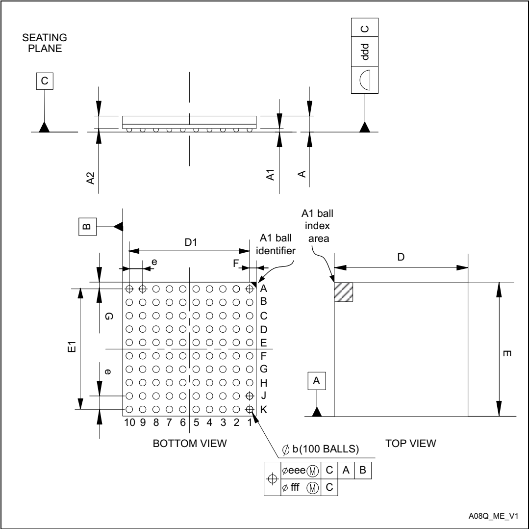
Figure 66. TFBGA100 - outline
