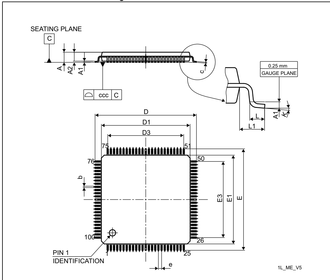
Figure 68. LQFP100 - outline
