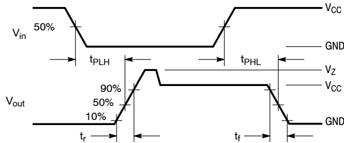
Figure 1. Switching Waveforms
