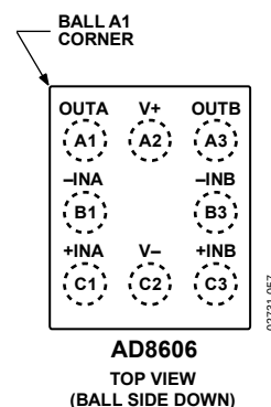
Figure 2. 8-Ball WLCSP (CB Suffix)
