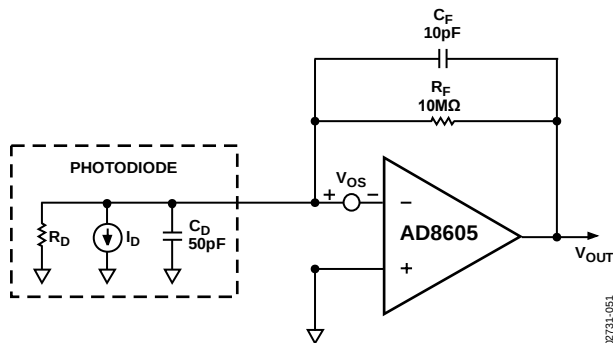
Figure 52. Equivalent Circuit for Photodiode Preamp
