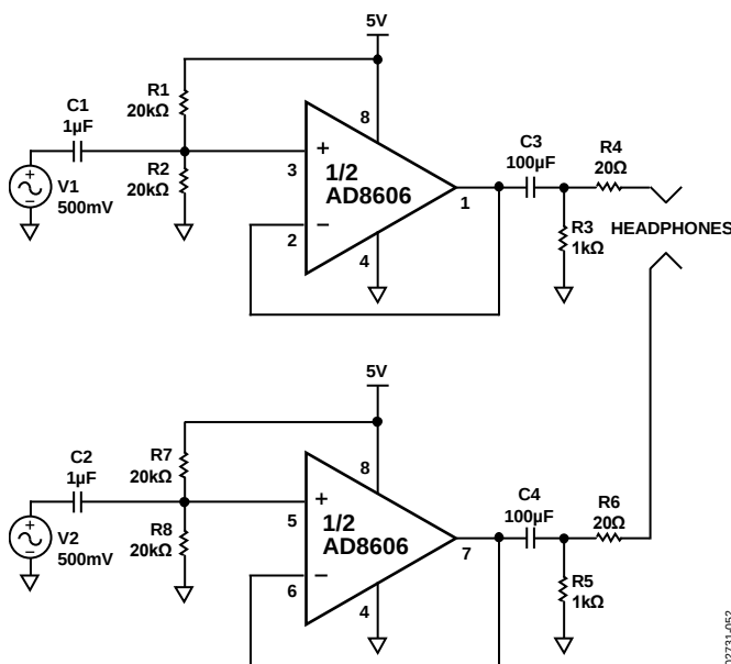
Figure 53. Single-Supply Headphone/Speaker Amplifier
