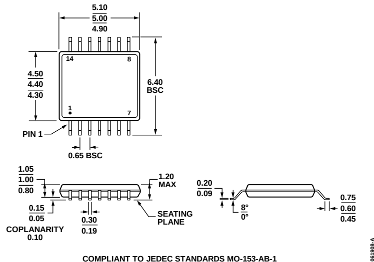
Figure 64. 14-Lead Thin Shrink Small Outline Package [TSSOP] (RU-14)
