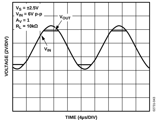
Figure 44. No Phase Reversal
