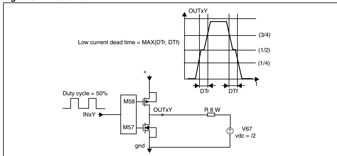
Figure 6. Test circuit 1
