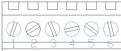
Figure 13: RS422 Header
