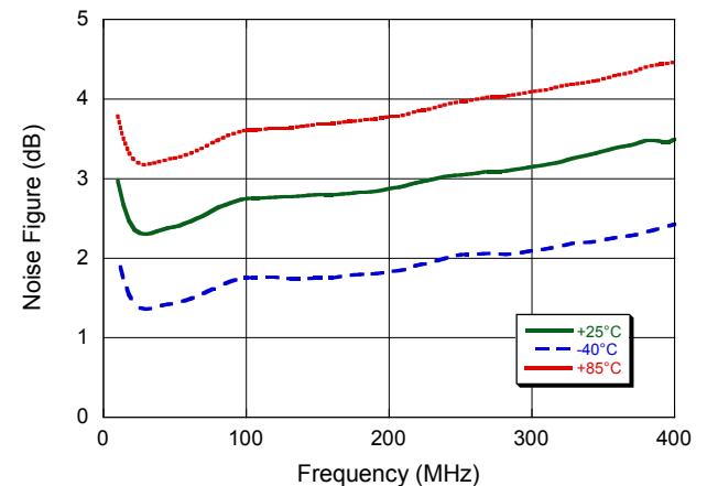
Noise Figure
