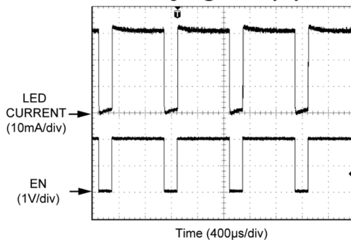
PWM Signal @ 80% Duty Cycle
