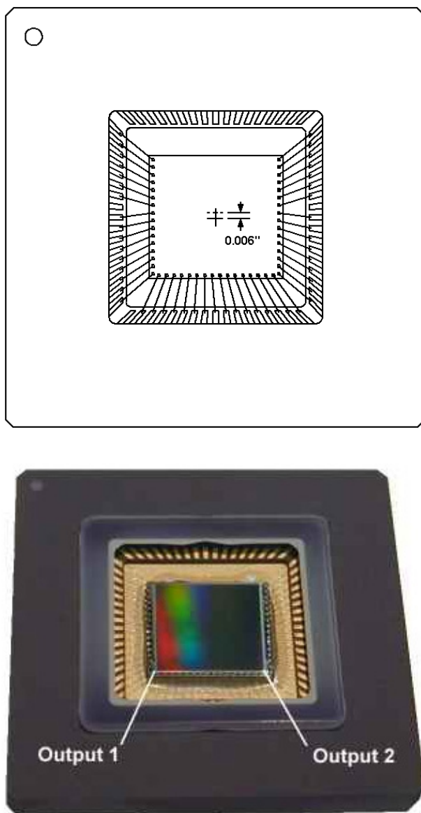
Figure 3. Pin 1 Location
