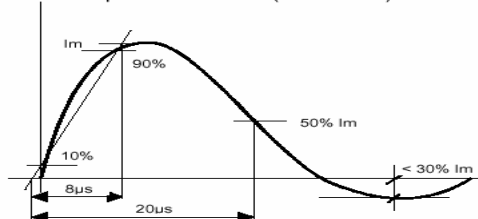
Wave shape "Short circuit" (Current Isc)
