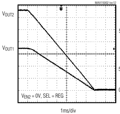
RATIOMETRIC SHUTDOWN
