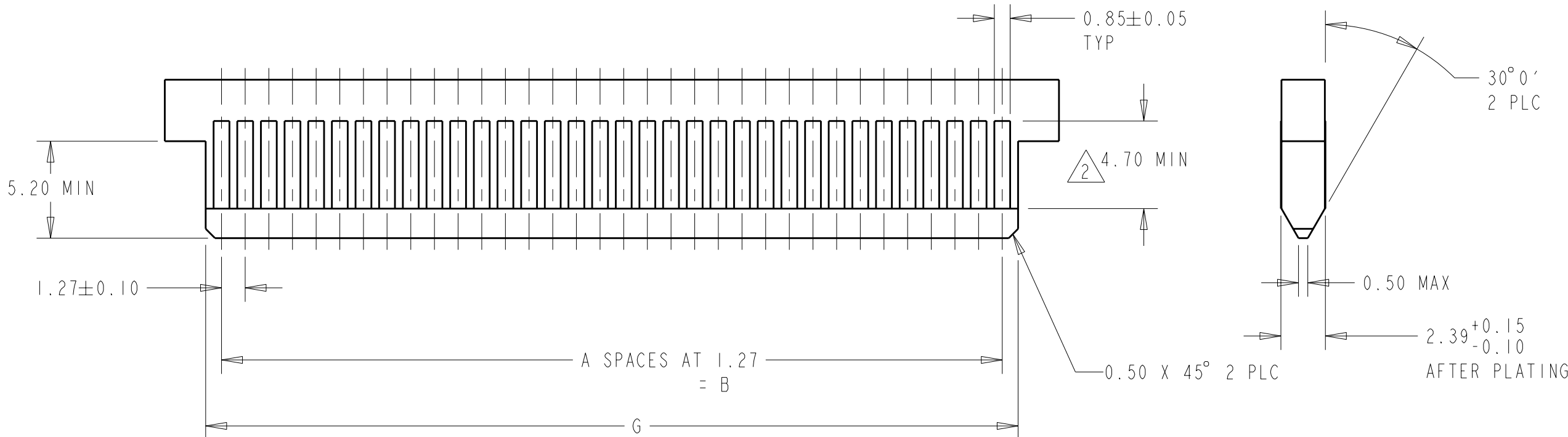
RECOMMENDED P.C.B. LAYOUT (CARD EDGE)
