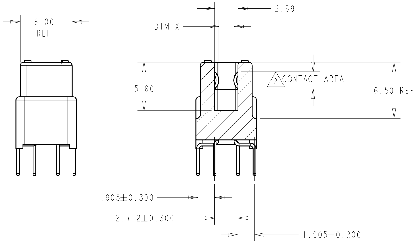
SECTION X-X
