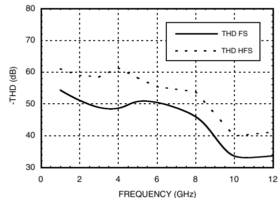
Hold-Mode THD vs. Frequency & Input Power @ f_{clk} = 4 \text{ GHz} @ 0 dBm
