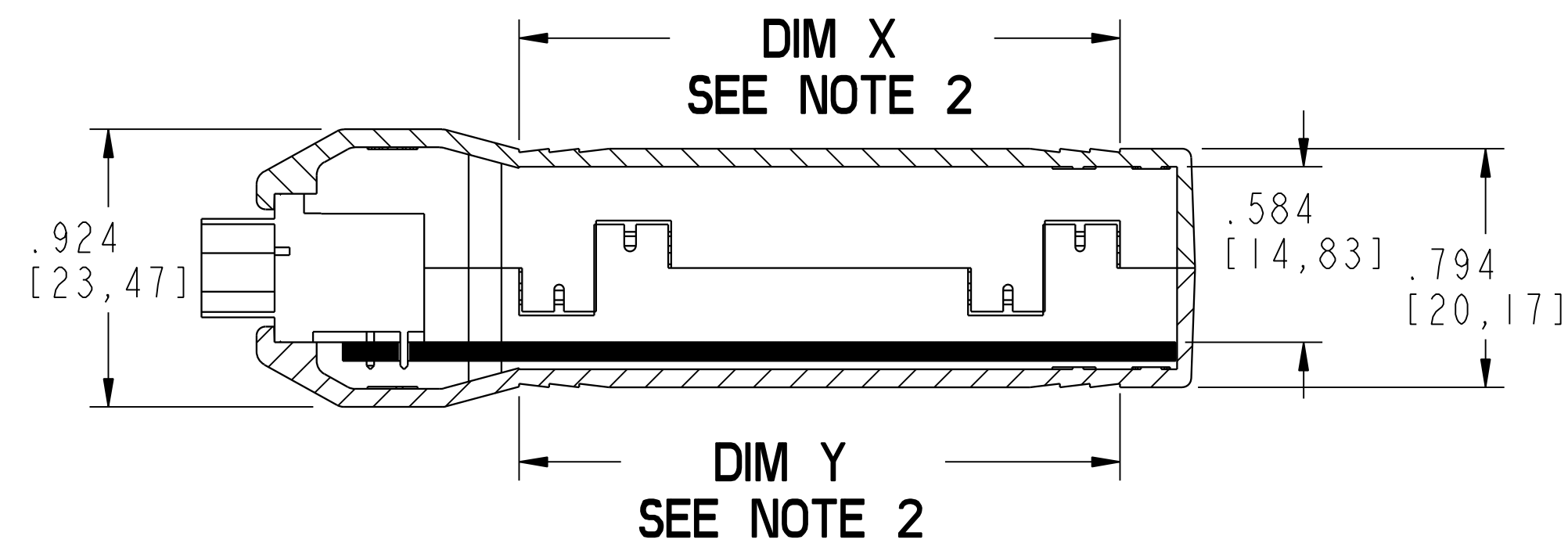
SECTION C-C
