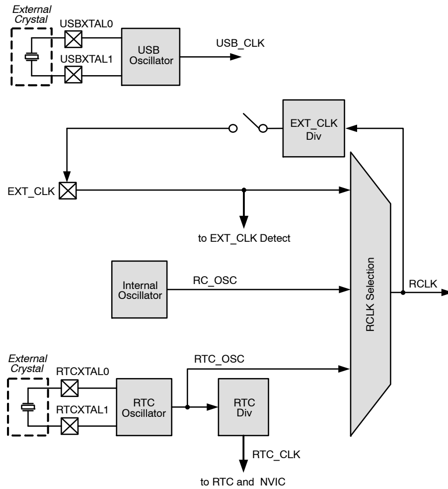
Figure 25. Clocking
