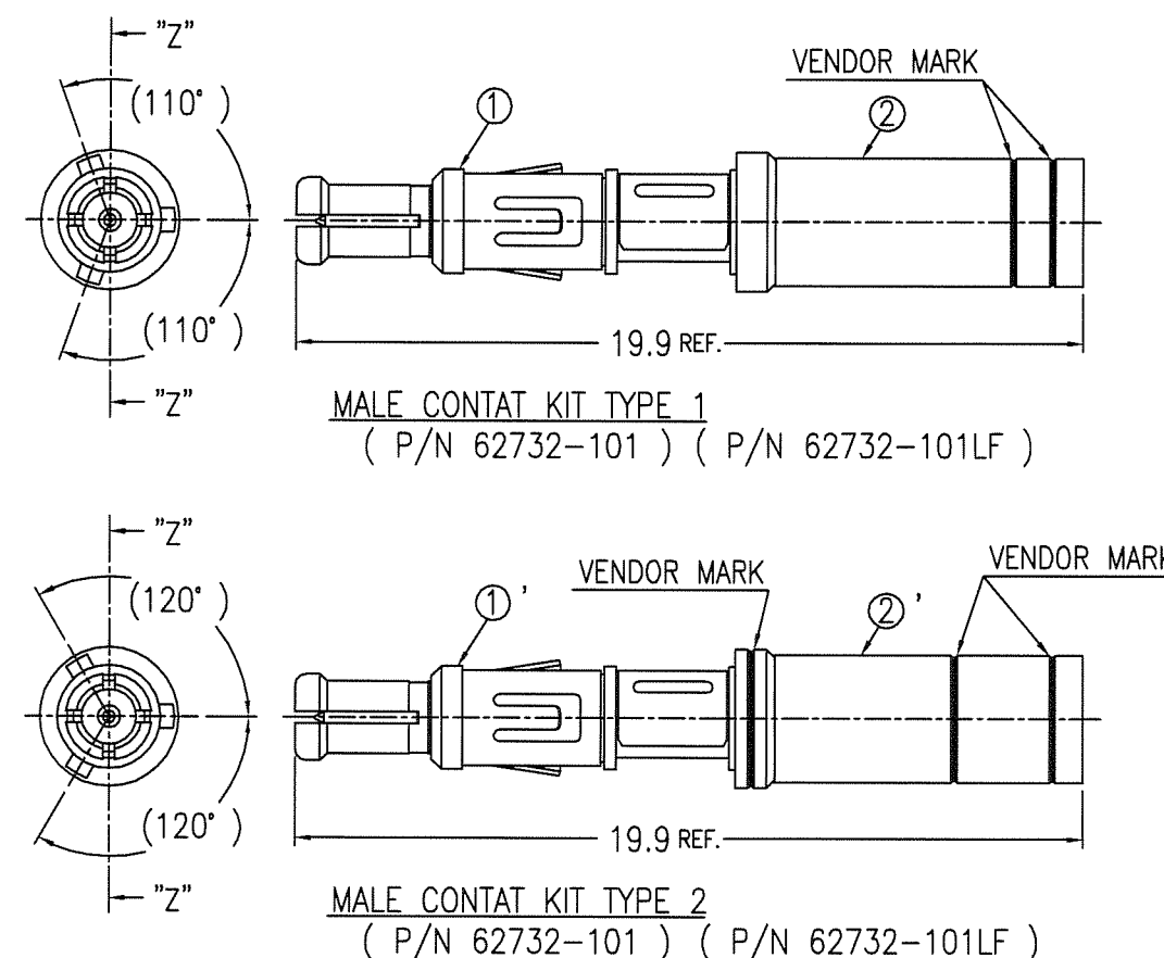
②' CLIMP SLEEVE ( P/N 62734-101B ) ( P/N 62734-101BLF )
