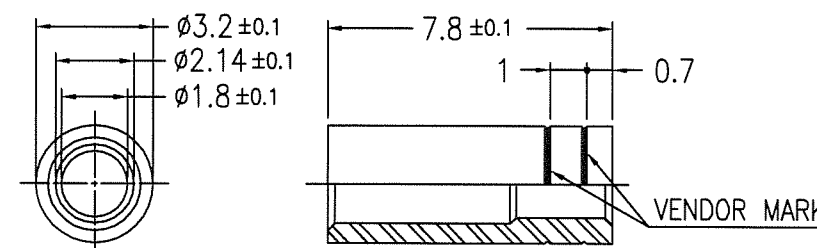
② CLIMP SLEEVE ( P/N 62734-101A ) ( P/N 62734-101ALF )
