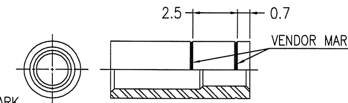
②' CLIMP SLEEVE ( P/N 62734-101B ) ( P/N 62734-101BLF )
