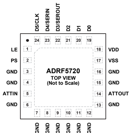
Figure 4. Pin Configuration
