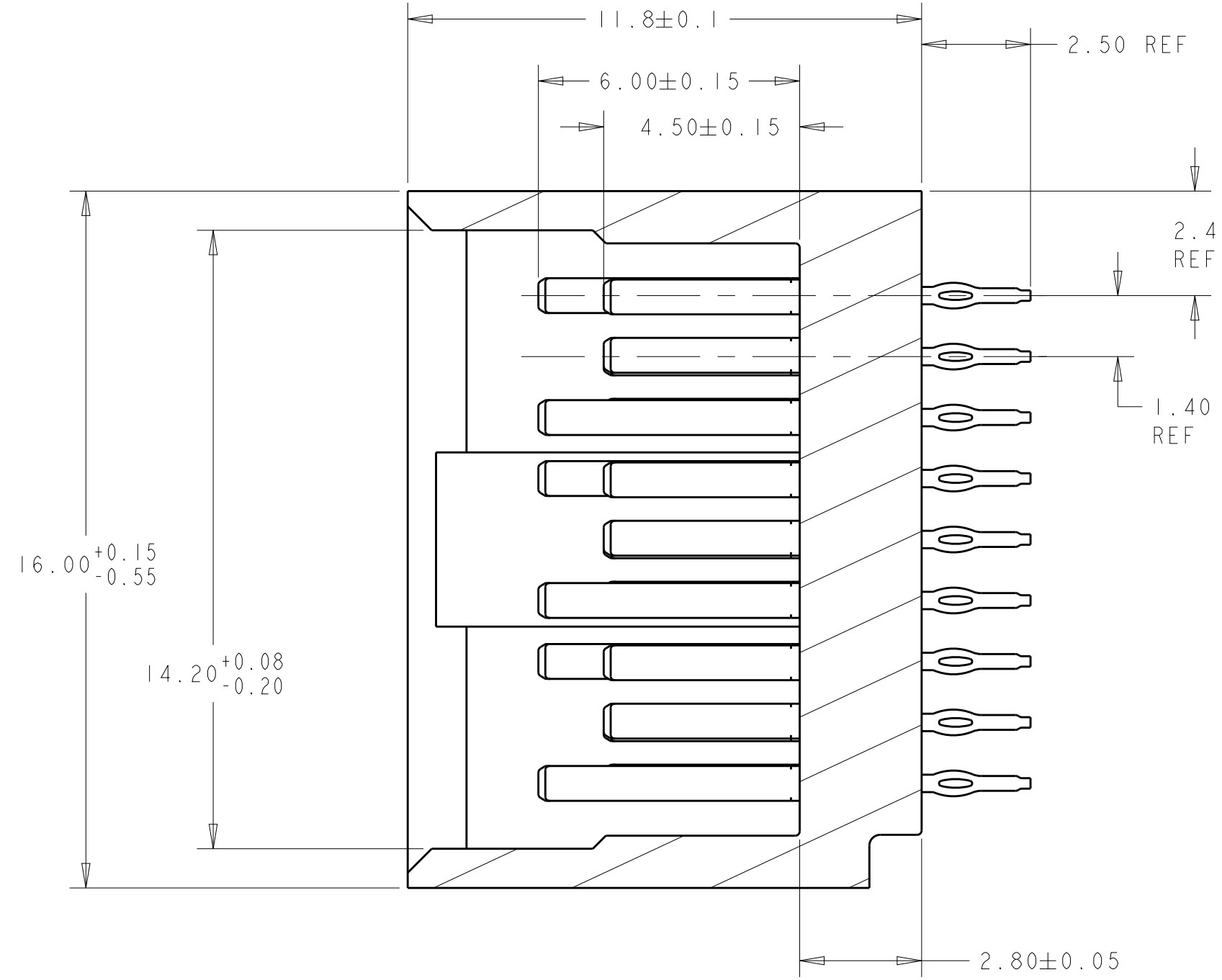
SECTION W-W
