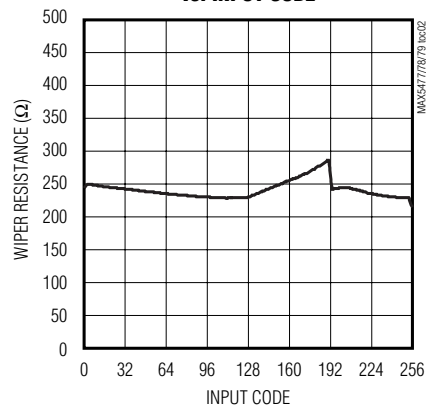
WIPER RESISTANCE vs. INPUT CODE
