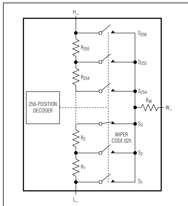
Figure 2. Potentiometer Configuration
