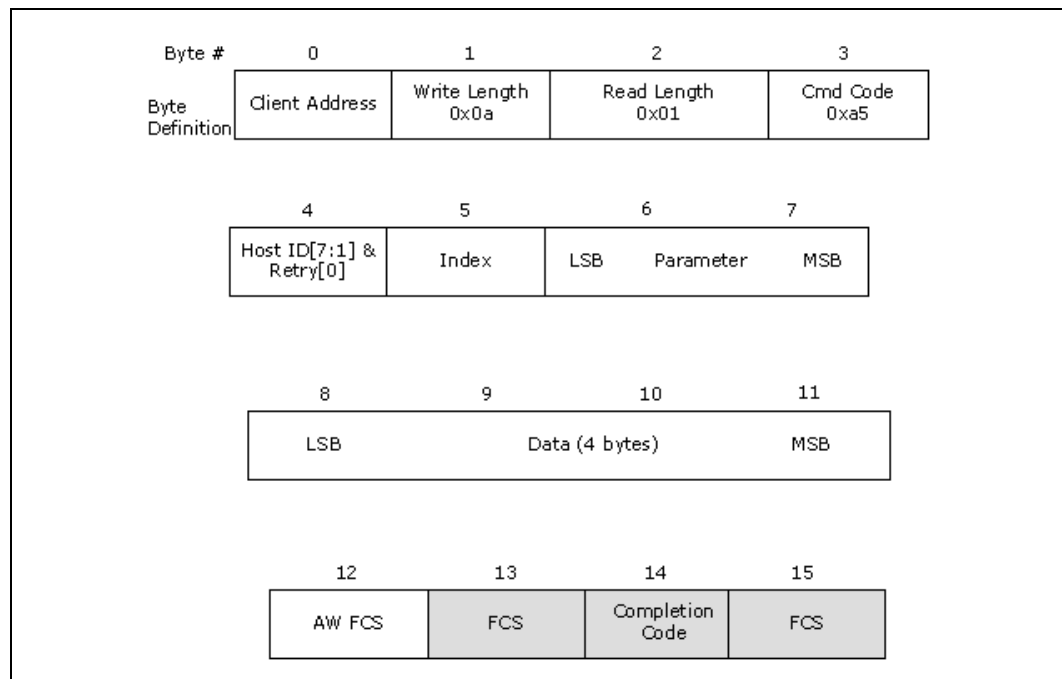
Figure 2-11. WrPkgConfig()
