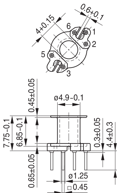
Hole arrangement View in mounting direction
