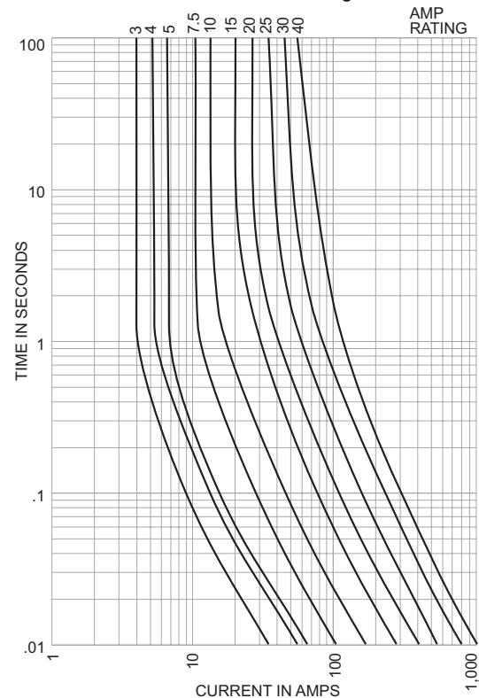
Time-Current Characteristic Curves - Average Melt
