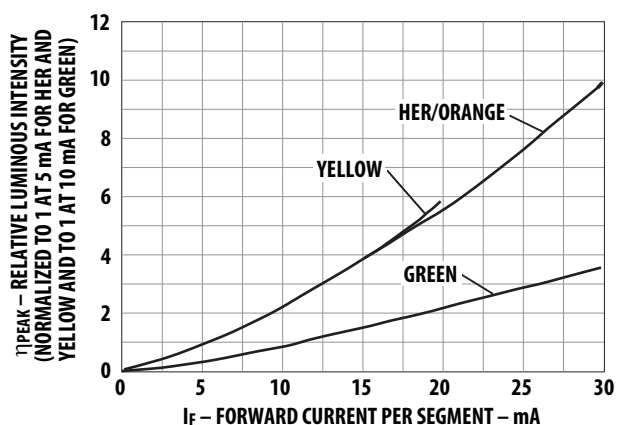
Figure 10. Relative Luminous Intensity vs. DC Forward Current.
