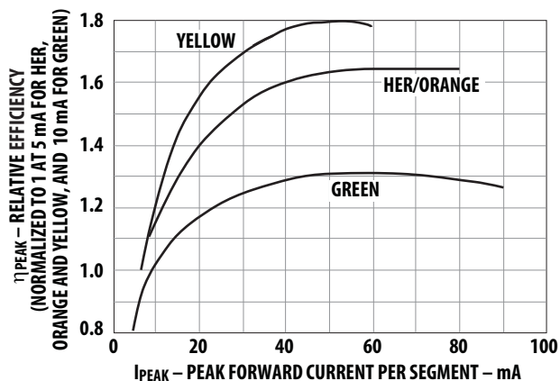
Figure 11. Relative Efficiency (Luminous Intensity per Unit Current) vs. Peak Current.
