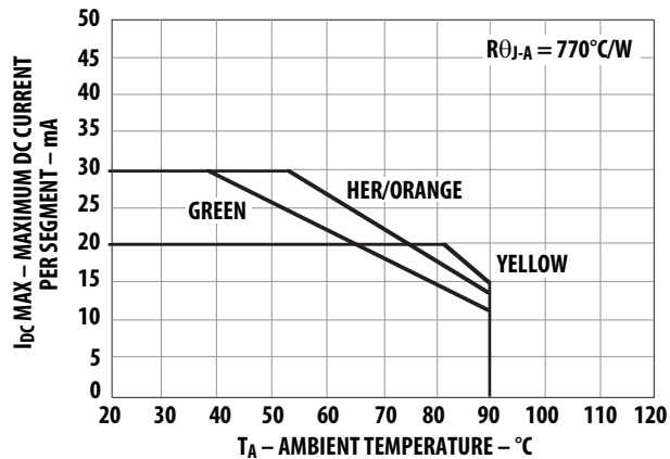
Figure 8. Maximum Allowable DC Current vs. Ambient Temperature.
