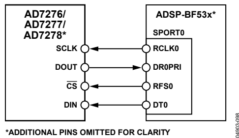
Figure 36. Interfacing with ADSP-BF53x
