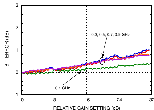
Bit Error vs. Relative Gain
