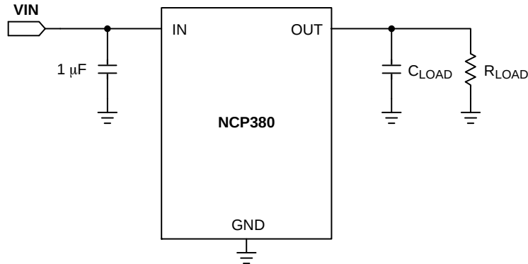
Figure 3. Test Configuration
