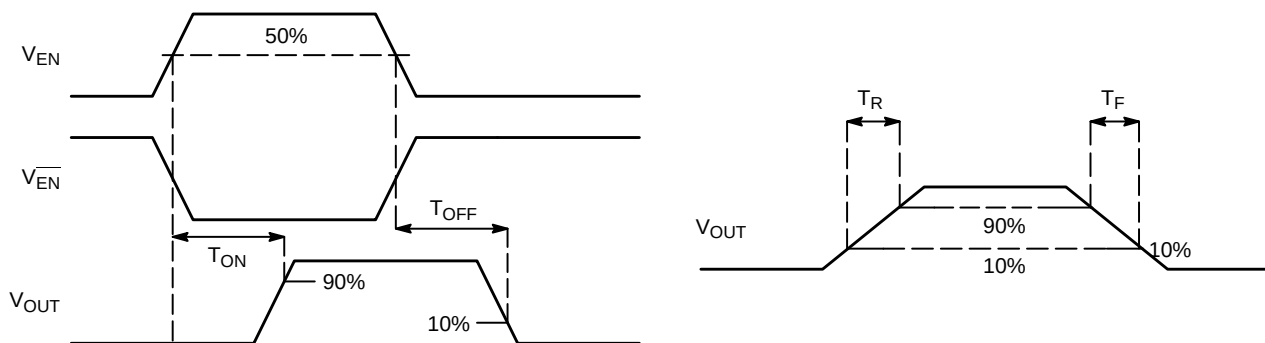
Figure 4. Voltage Waveform
